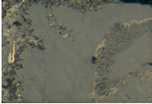
Structured tenuicutinite [c] in particle cut at an angle close to the bedding plane. (scale is 330 microns on long axis)
