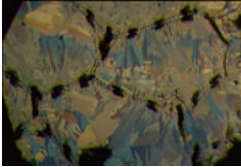
Massive marcasite overgrowth of plant cell structure. (Crossed polars) (scale is 330 microns on long axis)
