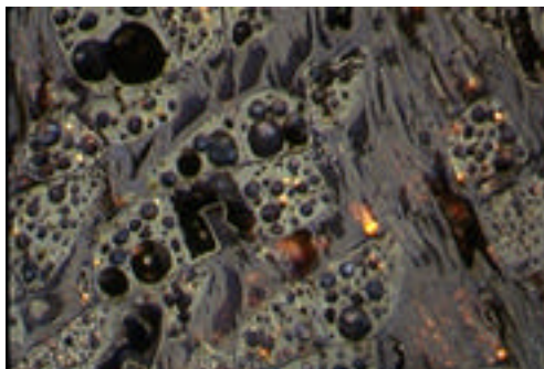
High-reflectance vesicular phlobaphinite (p) in texto-ulminite (t) matrix. (scale is 330 microns on long axis)
