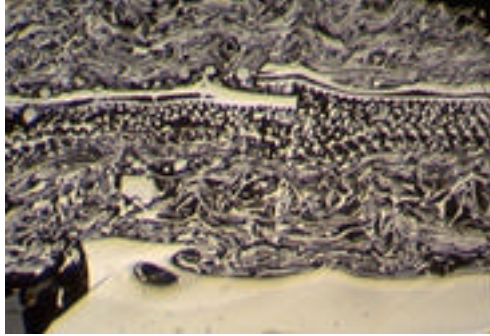
Broken fusinized cell walls (bogen structure) with variety of wall thicknesses and orientations. (scale is 330 microns on long axis)
